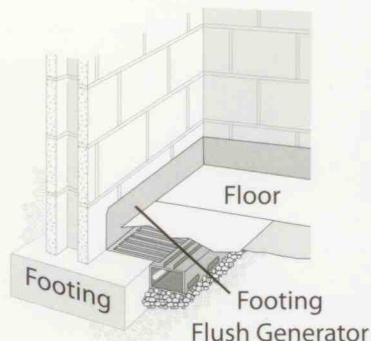
FOOTING FLUSH W/FLOOR
